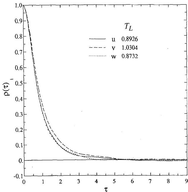
FIG. 14. Forced turbulence: velocity autocorrelations \rho(\tau) against time lag (\tau) , for the case F22 (conditions: N=32 , TS13, k_{\max}\eta=1 ). Calculated integral time scales ( T_L ) as indicated.
