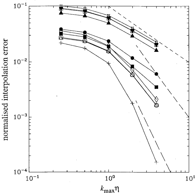
FIG. 2. Normalised interpolation error on velocity field specified by Pao's spectrum, against k_{\max}\eta , using a 32^3 grid. Interpolation schemes are identified by symbols: \Delta OPT15; \circ OPT13; \blacksquare OPT11; \bullet OPT9; \square OPT8; \diamond TS13; \blacktriangle TS9; \nabla TS8; \blacktriangledown linear; + splines; ---, --, —: lines of slopes -1 , -2 , -3 , respectively.
