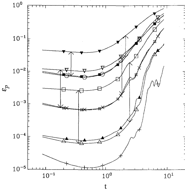
FIG. 5. Frozen turbulent velocity field (Pao's spectrum): averaged normalised rms error in particle displacement ( \epsilon_p ) against time ( t ). Grid sizes and interpolation schemes: \blacksquare N=32 , TS13; \circ N=32 , OPT13; \blacktriangledown N=32 , linear; \times N=64 , TS13; \square N=64 , OPT13; \nabla N=64 , linear; \triangle N=128 , TS13; \blacktriangle N=128 , OPT13; \square N=128 , linear; + N=128 , splines.
